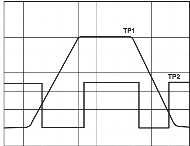
X-Axis = 0.2 ms/Division Figure 14. V_{CC} vs Output Waveform 1
