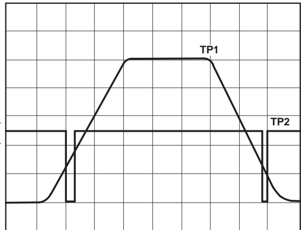
X-Axis = 0.2 ms/Division Figure 16. V_{CC} vs Output Waveform 2
