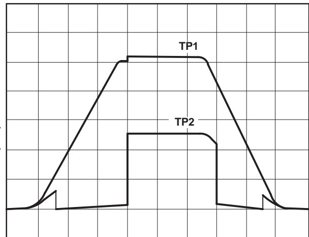
X-Axis = 0.2 ms/Division Figure 18. V_{CC} vs Output Waveform 3
